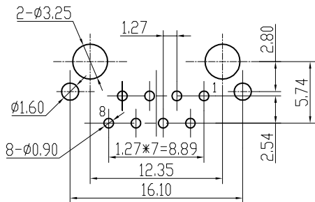
Pc Board Layout T=1.6mm Component Side Shown Tolerances ± 0.05
